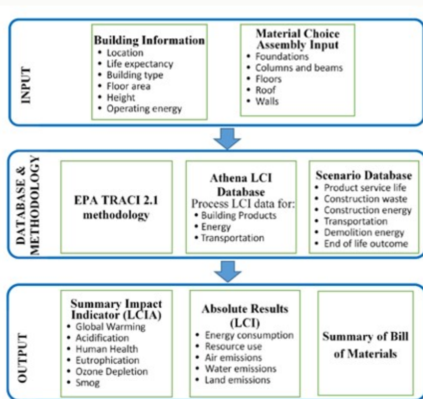
Fig.6 Athena Impact Estimator for Buildings (IE4B) calculation process based on ASMI (2019).
